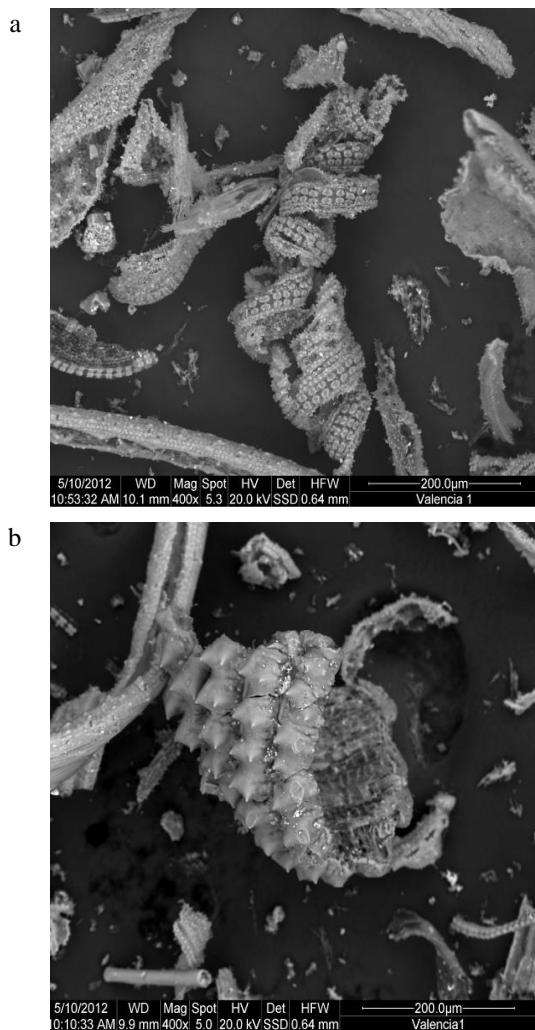
Figure 2: ESEM for two different zones of ash samples
