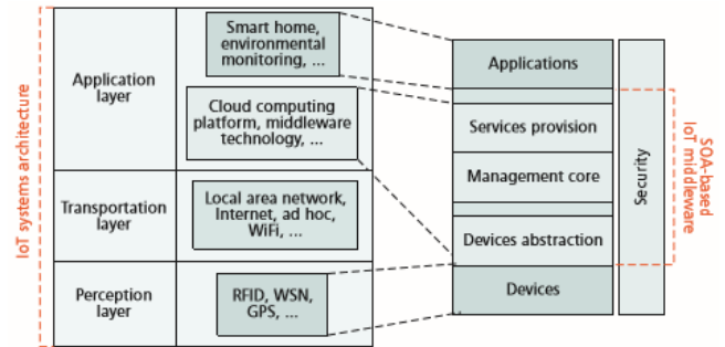
Fig. 8. SOA-middleware architecture[5]
