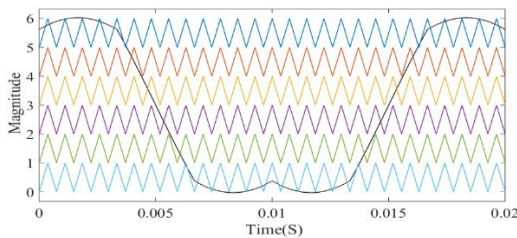
a) PDSVPWM
