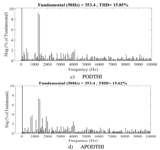
Figure 8. Harmonic analysis of DCMLI for different THI techniques
