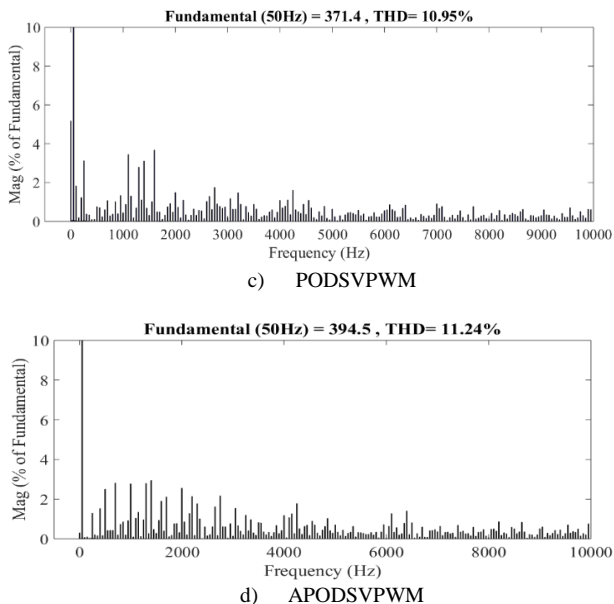
Figure 9. Harmonic analysis of DCMLI for different SVPWM techniques
