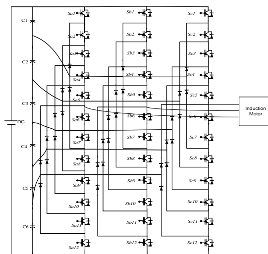
Figure 1. 7-level Diode Clamped Multilevel Inverter
