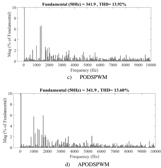
Figure 7. Harmonic analysis of DCMLI for different SPWM techniques
