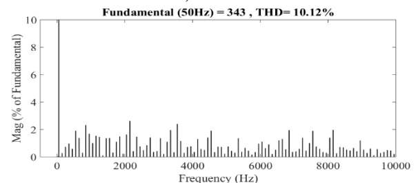
b) PDSPWM- Trapezoidal
