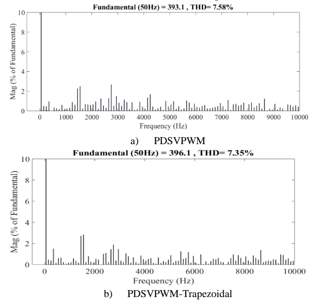
b) PDSVPWM-Trapezoidal
