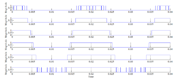
Figure 6. Gate pulses for SVPWM technique
