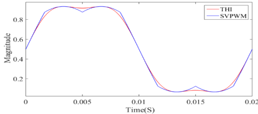
Figure 4. Comparison between reference signals of THI and Modified SVPWM
