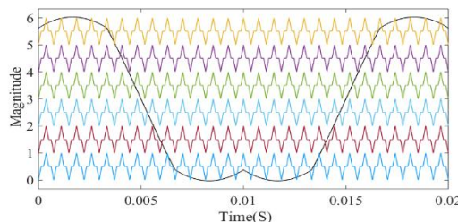
d) PDSVPWM- Trapezoidal
