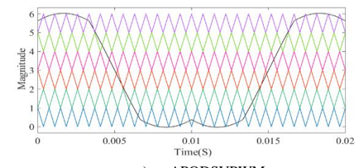
c) APODSVPWM
