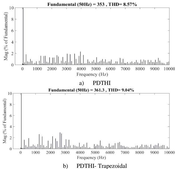
b) PDTHI-Trapezoidal
