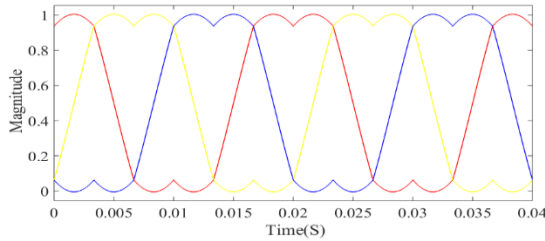
Figure 3. Reference signals for Modified SVPWM
