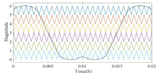
b) PODSVPWM
