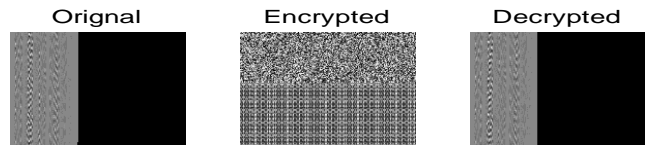
Figure 3. Image Encrypted/Decrypted.
