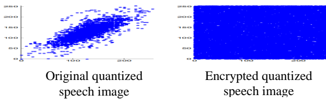
Figure 9. Correlation comparison.
