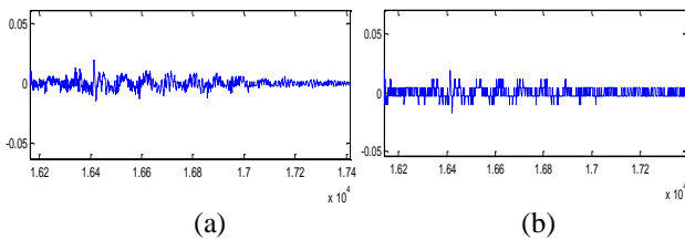
Figure 8. The end of the original speech signal (Zoomed), (b) the same region of the reconstructed speech signal after Decrypted and Dequantization (Zoomed).
