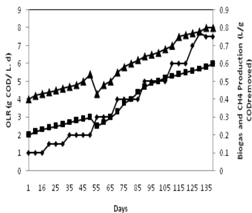
Figure 2: Biogas and CH 4 production in terms of OLR influence, where ♦ OLR (g COD/L), ■ CH 4 production (L/g CODremoved), ▲ Biogas production (L/g CODremoved).
