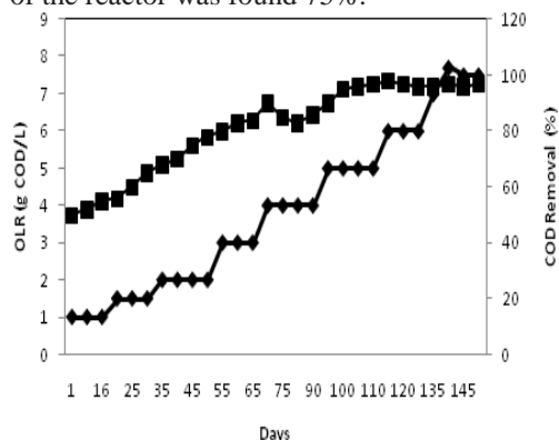
Figure 1: COD removal efficiency in terms of OLR influence, where \blacklozenge OLR (g COD/L), \blacksquare COD removal %
