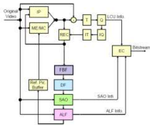
Figure 2 Block Diagram of HEVC Encoder with Fast Bilateral Filter.
