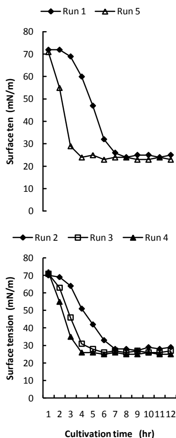
Figure 2. Pattern of surface tension of cell-free culture broth of exponentially fed-batch fermentation runs.
