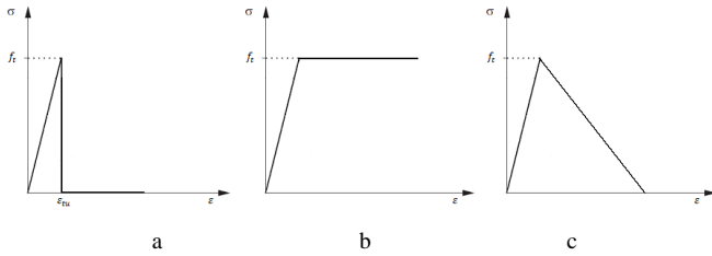
Figure 23. Tensile constitutive laws: (a) elastic-brittle, (b) elastic-plastic, (c) linear tension softening
