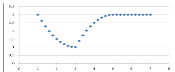
Figure 1. PNC modeling for nine reconstructed points between nodes.
