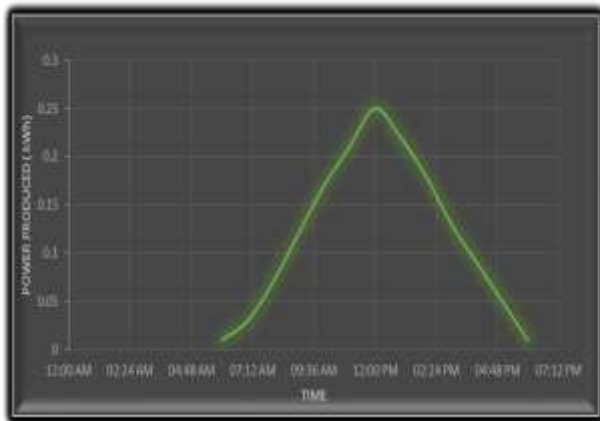
Graph 2: GRAPH REPRESENTING AMOUNT OF ELECTRICAL ENERGY PRODUCED PER DAY
