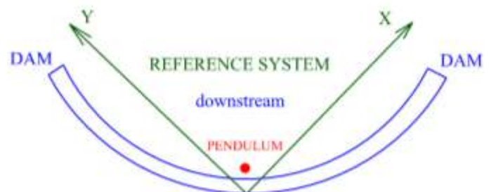
Figure 4. Pendulum reference system in La Cohilla Dam.
