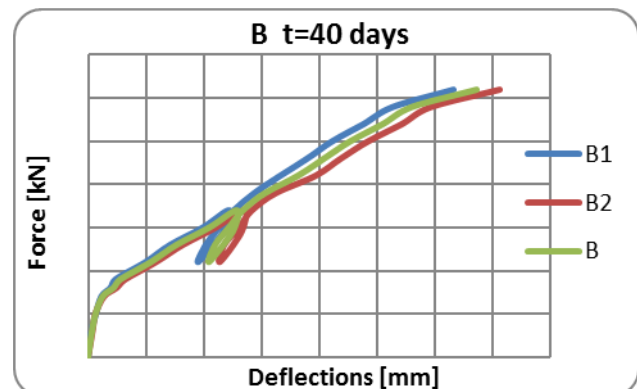
Chart 4 Comparison of deflection diagrams series B t = 40 days [1]
