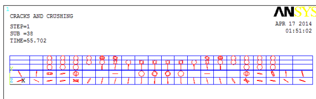
Figure(13): Shear cracks of pre-slab S2.
