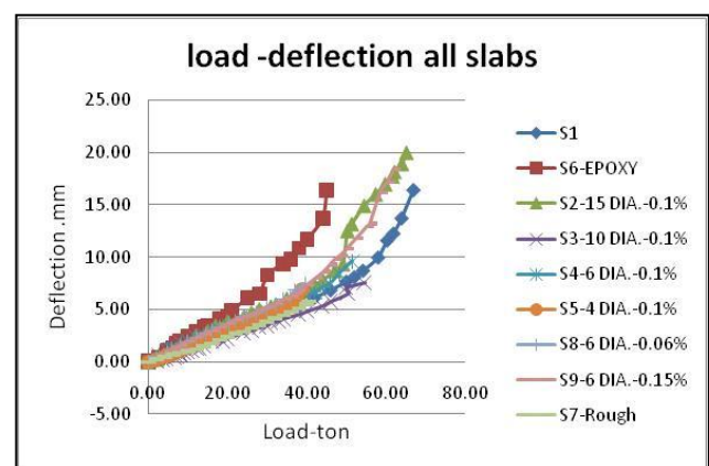
Figure (11): Load Deflection Curves.
