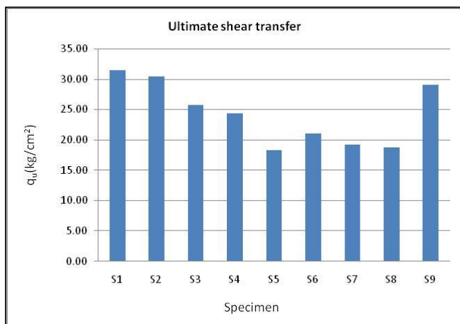
Figure (10): Ultimate shear transfer for the tested specimens.
