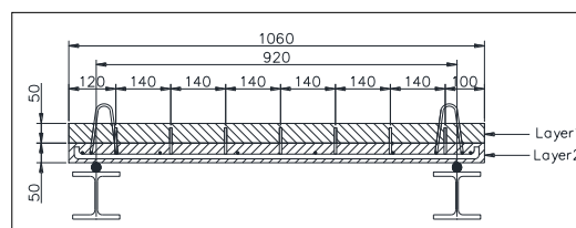
Figure (1b): Arrangement of shear dowels for pre-slabs S2-S5.
