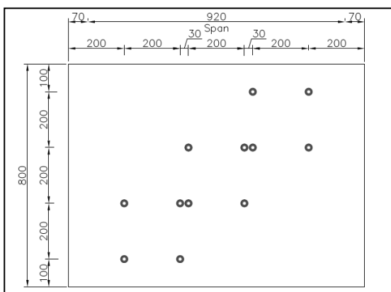
Figure (3): Demic points under uniformly distributed load.
