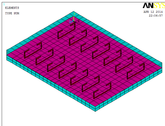
Figure(12): Finite element mesh for pre-slab S2.
