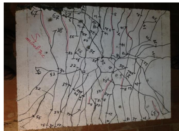
Figure (6): Crack pattern of slab S1.
