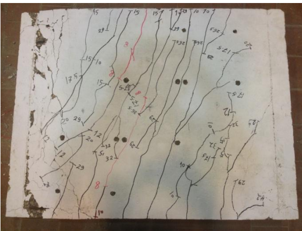
Figure(8): Crack pattern of slab S2.
