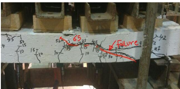
Figure (9): Shear failure of slab S2.
