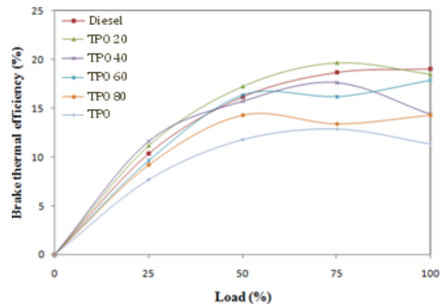
Fig. 4.2 Comparison of brake thermal efficiency with load
