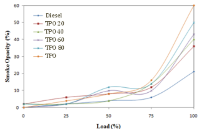
Fig. 4.6 Comparison of Smoke emissions with load
