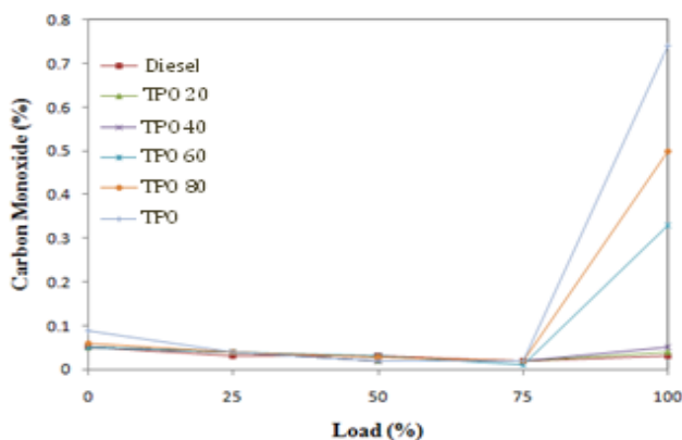
Fig. 4.4 Comparison of Carbon monoxide emissions with load
