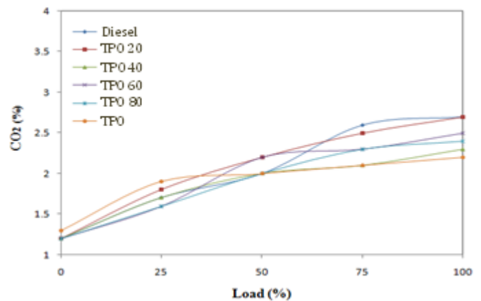
Fig. 4.5 Comparison of Carbon dioxide emissions with load
