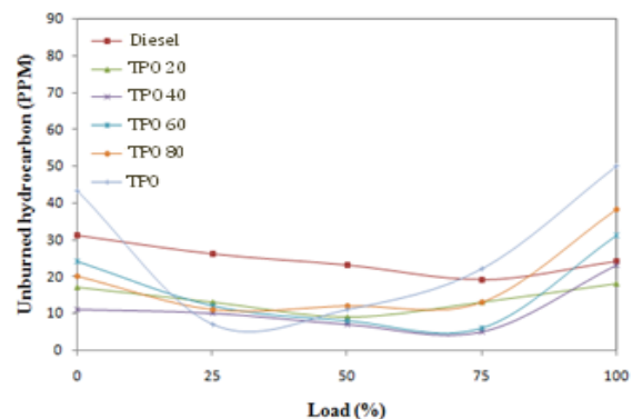
Fig. 4.3 Comparison of Unburned hydrocarbon emissions with load
