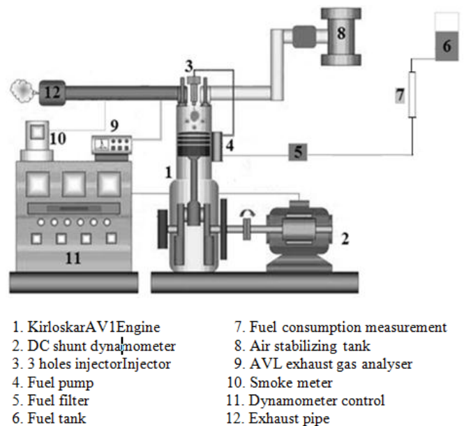
Fig. 3.1. Schematic of experimental setup
