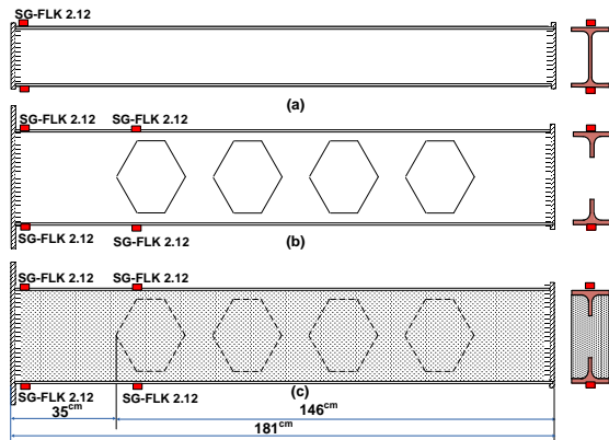
Figure 2. Beam test for the : (a) normal beam (nb), (b) castella (cb), (c) castella composite beam (ccb)
