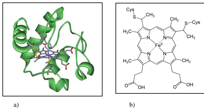
Fig. 13a,b: band model of cytochrome c with the prosthetic group heme-c as model a) and chemical structure of heme c with 4 pyrrole-rings in a porphyrin-ring (b) (source: Wikipedia)
