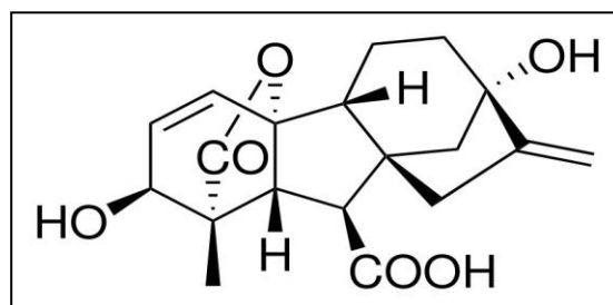
Fig. 1: chemical structure of gibberellic acid (source: Wikipedia)
