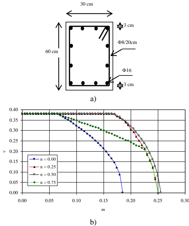
Figure 2. a) cross section; b) dimensionless shear v vs. bending moment m interaction strength domain for different values of specific axial force n
