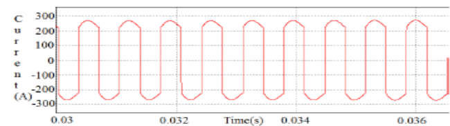
Fig. 4. Current waveforms
