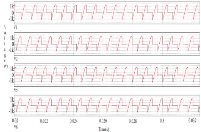
Fig. 2. Voltage across thyristor
