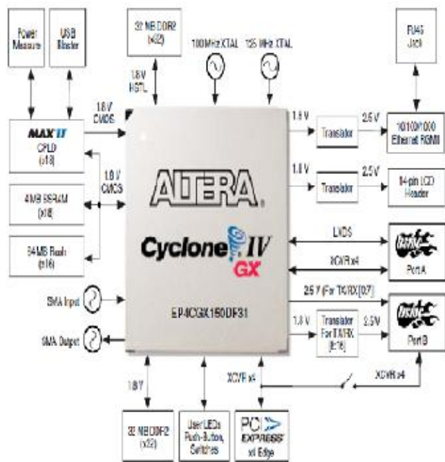
Fig. 9. FPGA controller
