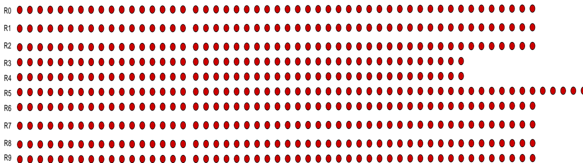
Fig. 7. The number of chip ID generation circuits on each row: R0-51, R1-51, R2-51, R3-44, R4-44, R5-56, R6-51, R7-51, R8-51, R9-51, R10-51
