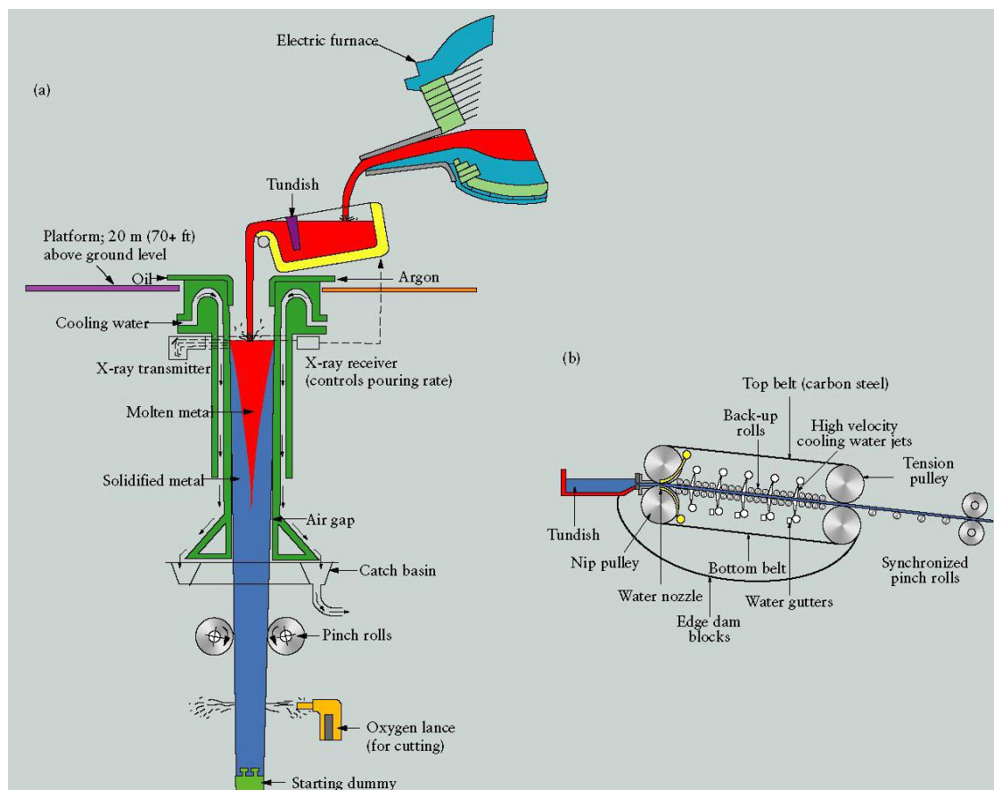
Figure-4 Continuous Casting Process with a starter bar
