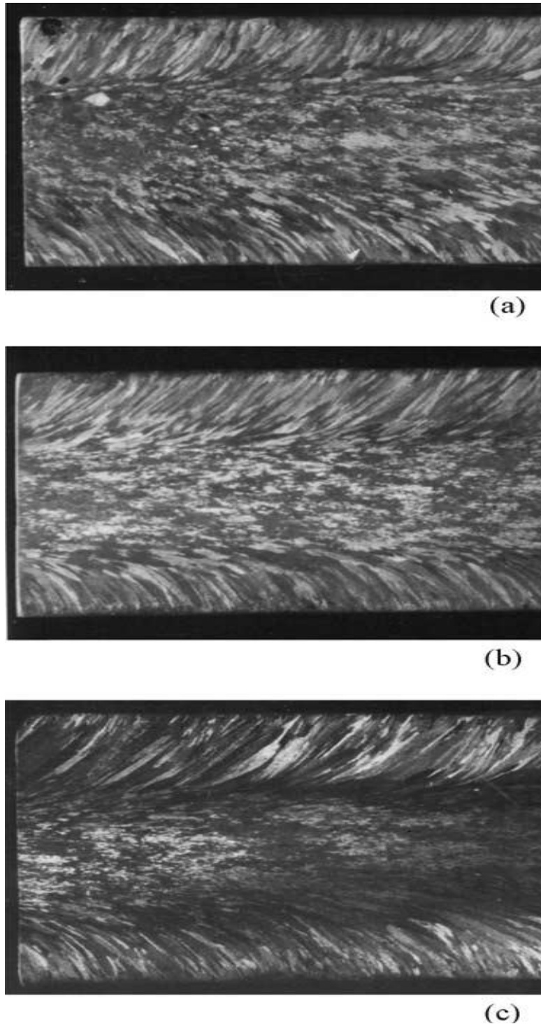
Figure-7 Macrostructure of continuously cast Al-1.2Li-0.8 Hf alloy ingot. (a) Top, (b) Middle and (c) Bottom parts [14]
