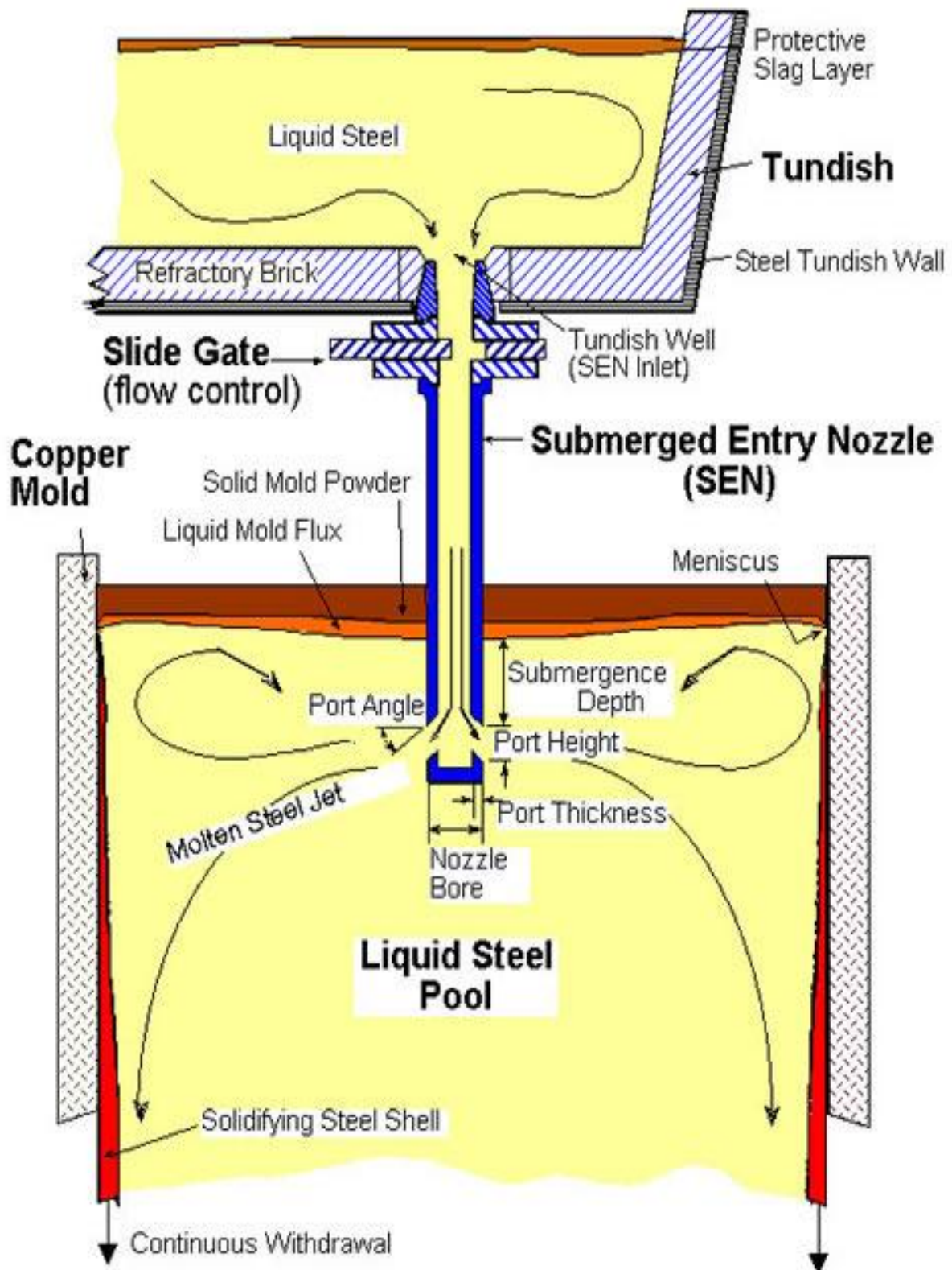
Figure-5(a) Mechanism of Continuous Casting Process
