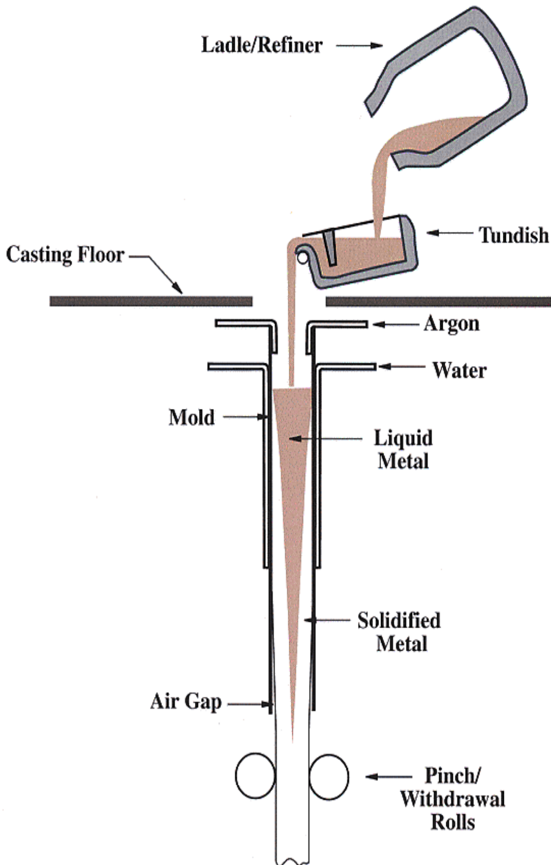
Figure-3 (a) Schematic Sketch of Continuous Casting Process
