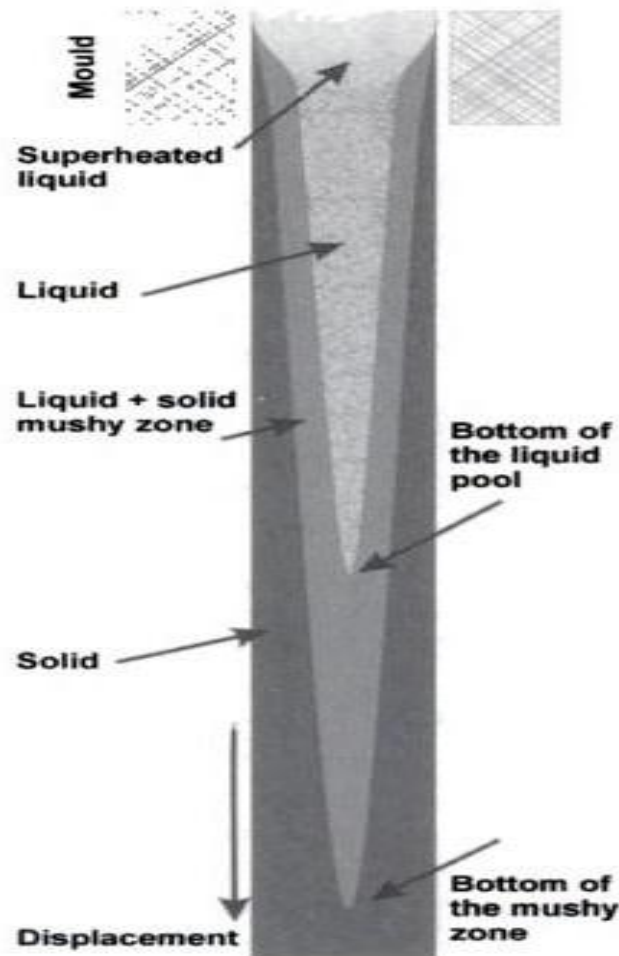
Figure-9 Schematic sketch of an axial section of a continuously cast ingot
