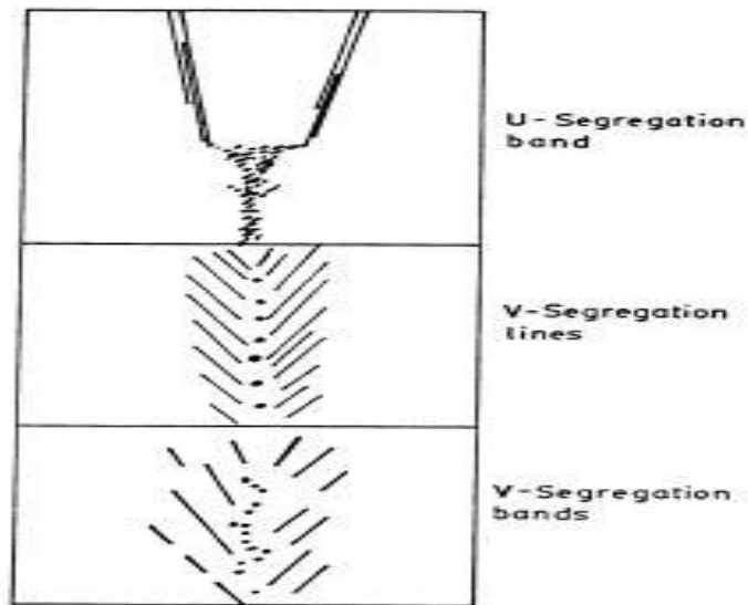
Figure-10 Features of macro segregation in longitudinal section of continuously cast billets [13]
