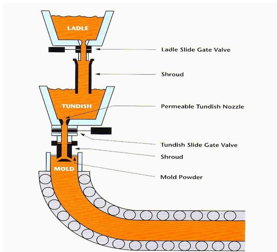
Figure-1 Schematic sketch to illustrate the principle of continuous casting process
