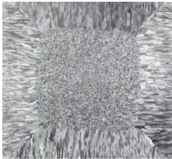
Figure-8 Macrostructure of a continuously cast stainless steel bloom
