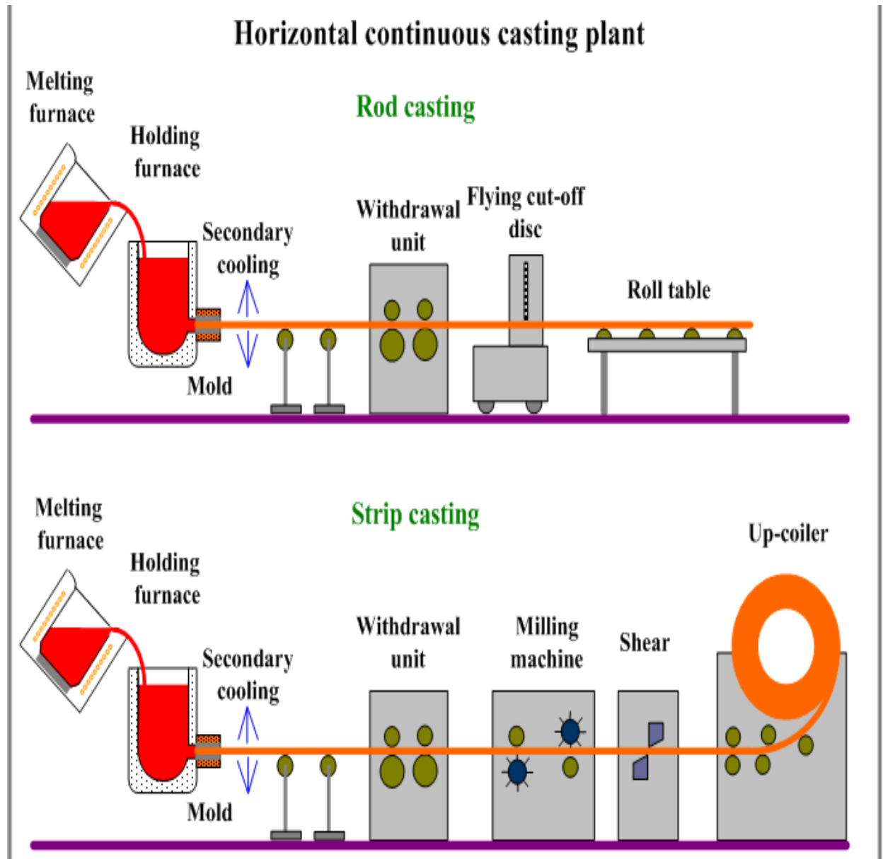
Figure-2 Horizontal continuous casting plant
