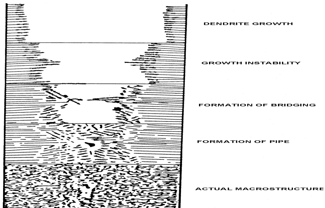
Figure-6 shows the macrostructure of a slab cast in a continuous casting machine [13]
