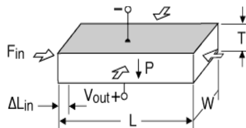
Fig.2.5Transverse (d31) generator
