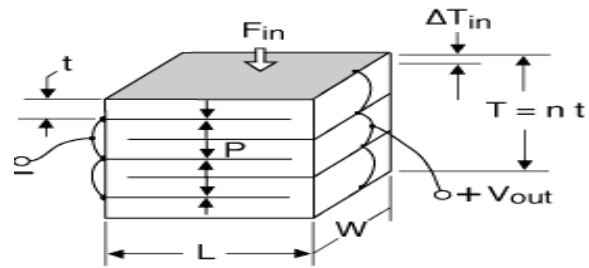
Fig2.6: Multi-Layer Stack Generator
