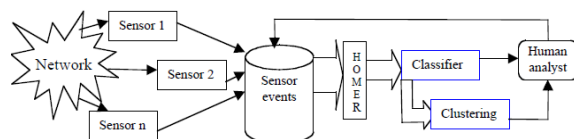
Fig 3 How ensors feed into overall intrusion detection system
