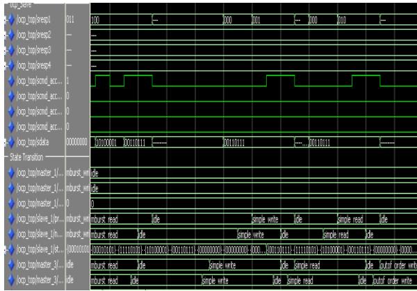
FIGURE5-SIMPLE TRANSACTIONS
