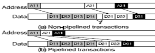
FIGURE4: Pipelined transactions
