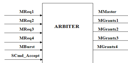
FIGURE1.1: OCP ARBITER
