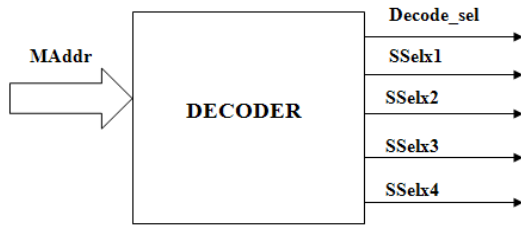
FIGURE 1.2: DECODER
