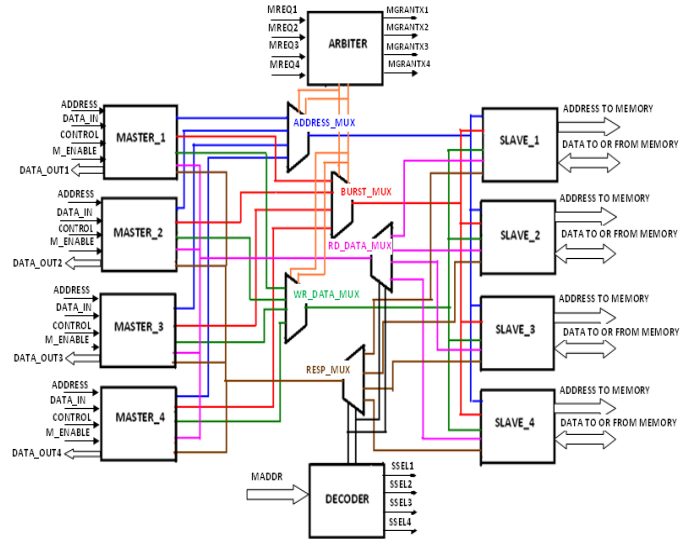
FIGURE1: Bus Architecture
