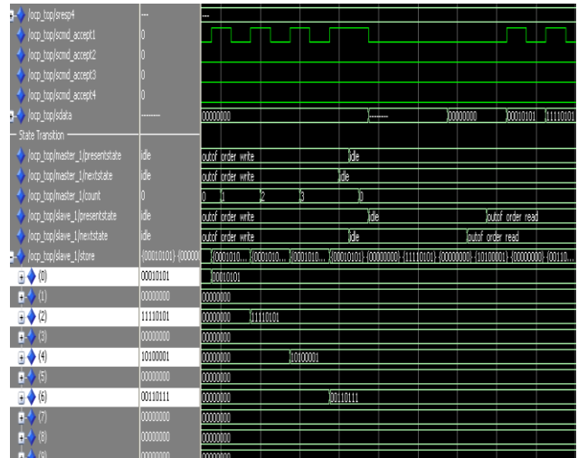
FIGURE 8 OUT OF ORDER TRANSACTIONS
