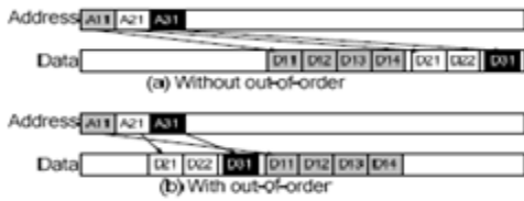
Figure 3.Out of order transactions
