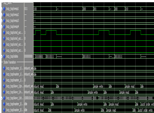
FIGURE7-PIPELINED TRANSACTIONS
