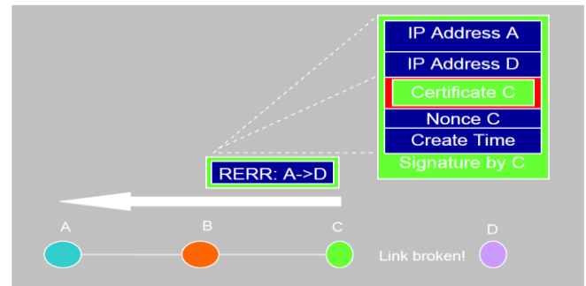
Figure 2: Route Maintenance
