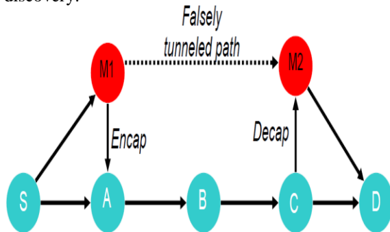
Figure 1 Wormhole Attack
