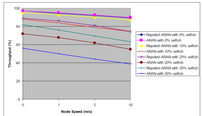
Figure 8: Effects of Selfish nodes on Network Throughput
