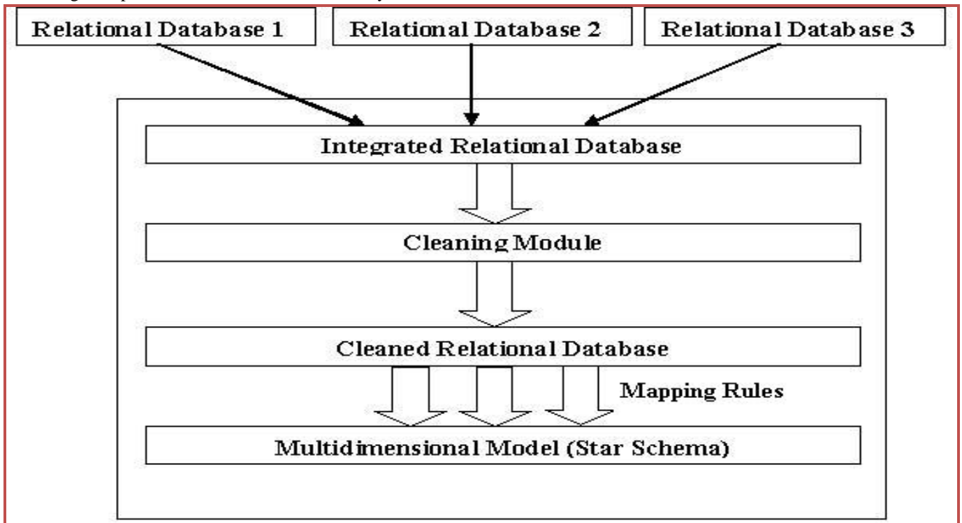
Figure 1. Proposed Framework
