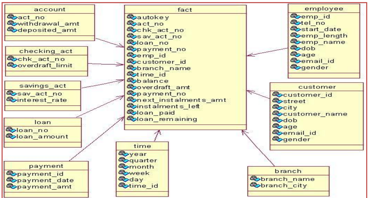
Figure 7. Star Schema
