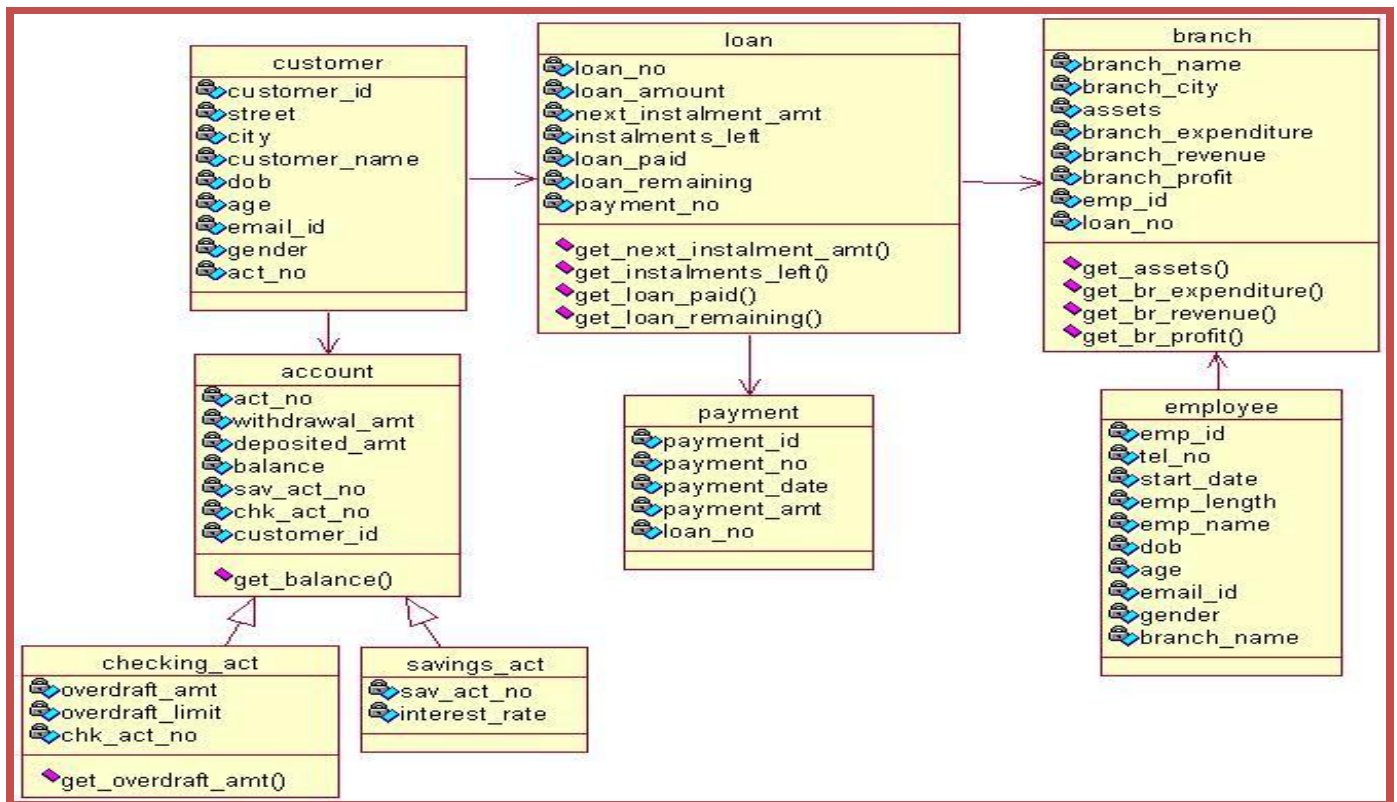
Figure 6. Bank Management System Class Diagram
