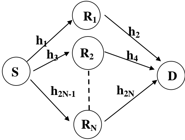
Fig. 2. N- branch dual-hop relay diversity links
