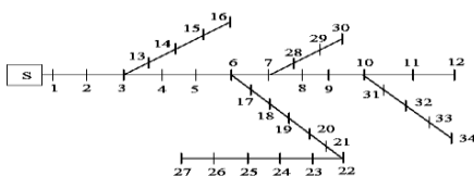
Figure 3. IEEE 34-Bus Test System
