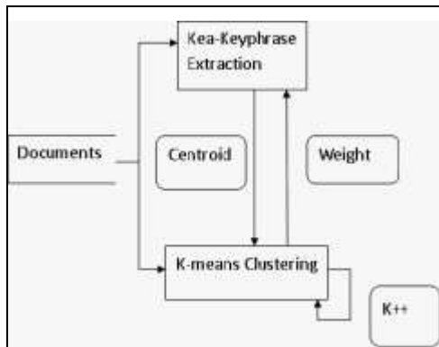
Fig 3 The process of Kea-means clustering
