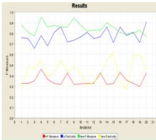
Fig 4 Result of Reuters dataset
