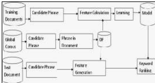
Fig 1 The training and extraction processes
